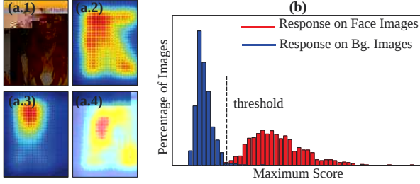
Figure 3. (a.1) Original image. (a.2)-(a.4) are averaged response maps in C5 of LNet c after pre-training (a.2), fine-tuning (a.3) and directly training from scratch with attribute tags but without pre-training (a.4). (b) Determine threshold.
